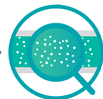
SILVER IONS
